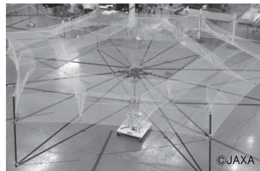
Photo 1 One module of the LDR.
