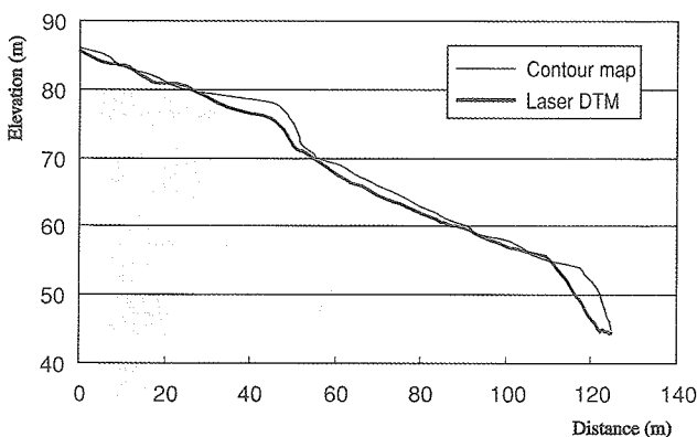
Fig. 11 Overlap of cross sections based on a photogrammetric contour map and laser DTM (Kawasaki sub-area).
