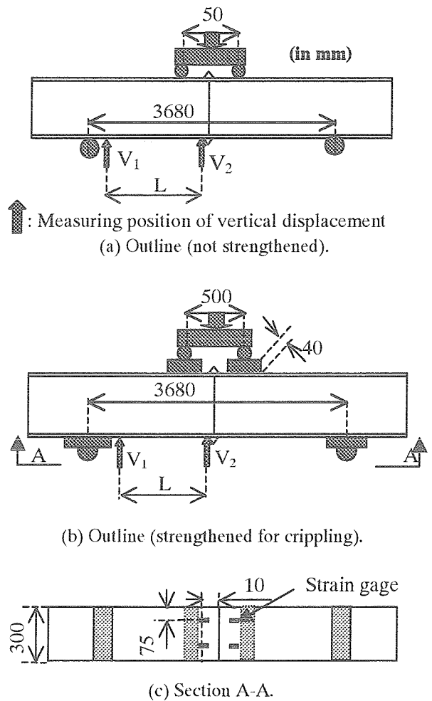
Fig. 3 4-point bending test for rolled H section welds.
