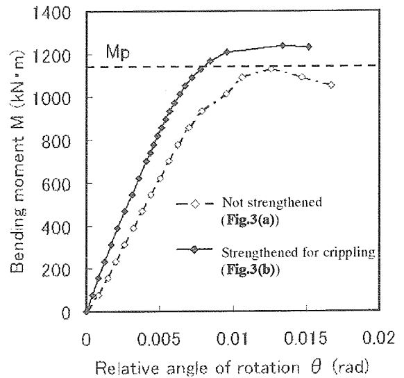
Fig.6 Bending moment M and relative angle of rotation \theta diagram at welded zone.
