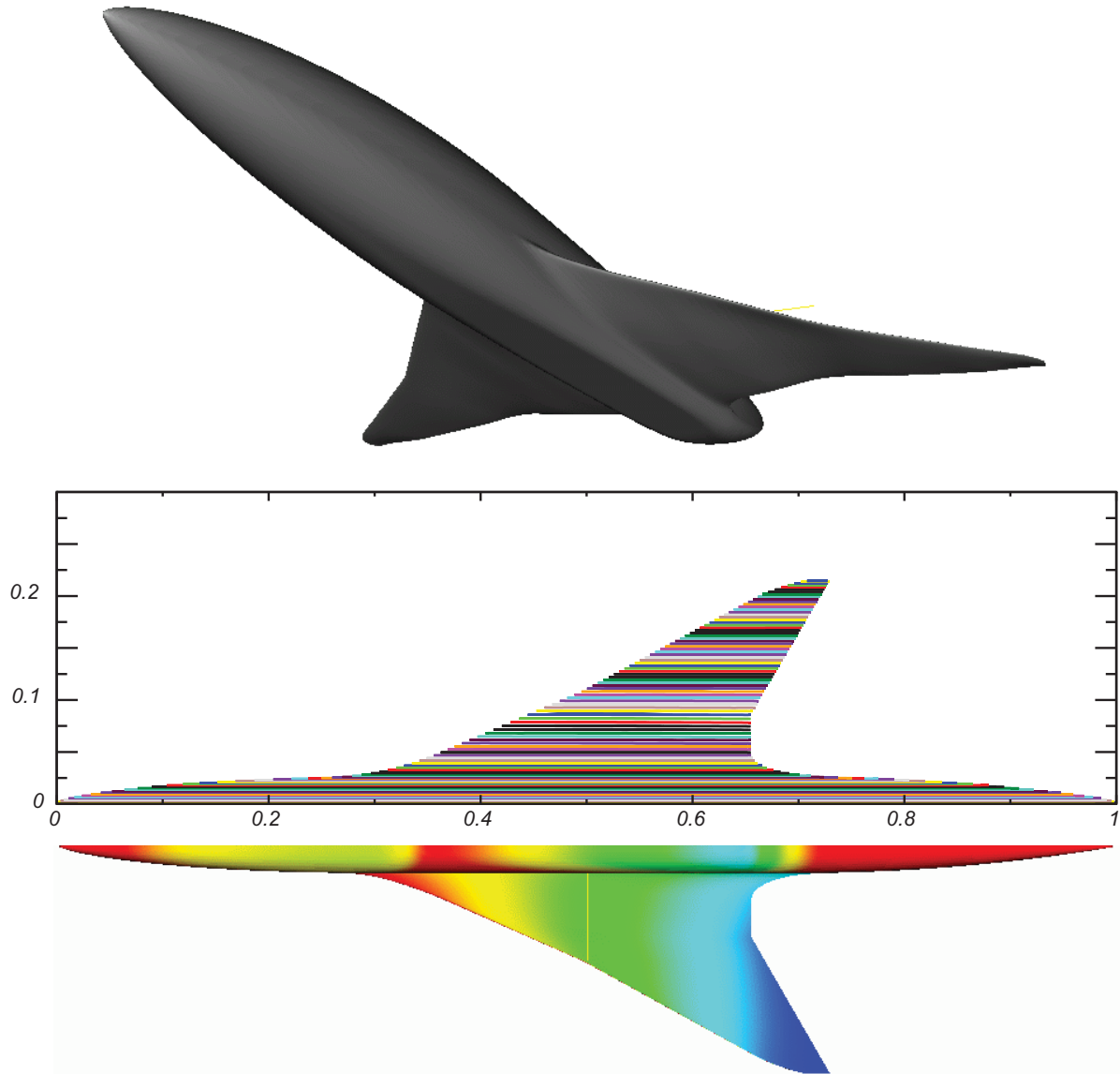
Figure 3. Wing-body configuration
