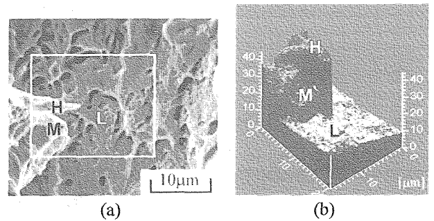
Fig. 7 Three-dimensional topography around the analysis point: (a) SEM micrograph, (b) DEM of the reconstructed fracture surface.
