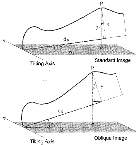
Fig. 2 Schematic illustration of stereo-photogrammetry.
