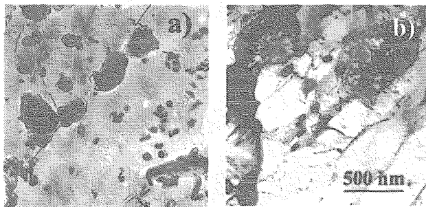
Figure 2 Size, morphology and distribution of carbide particles in the microstructure of original state: (a) TEM micrograph of carbon extraction replica and (b) TEM micrograph of thin foil.
