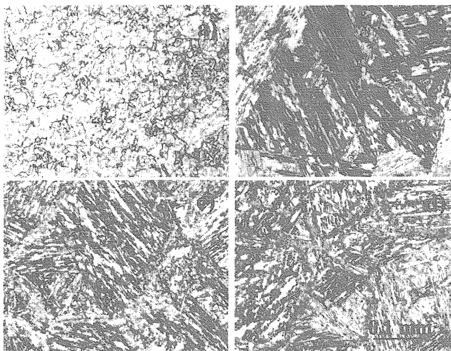
Figure 1 Characteristic microstructures of the investigated steel: (a) after rolling, normalizing and tempering (OR), (b) after 1 st welding cycle (state C), (c) after 2 nd welding cycle (state A), (d) after 3 rd welding cycle (state A3).
