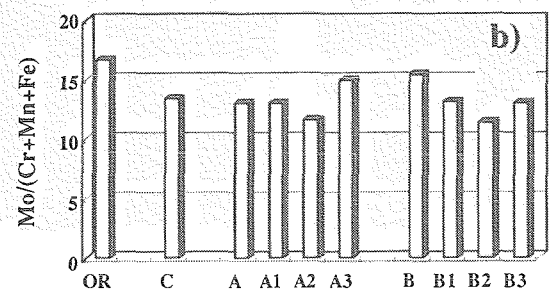
Figure 9 Changes in metal composition of identified carbides (atomic contents of Cr, Mn, Fe, and Mo were taken into account) in analyzed states: (a) Fe/(Cr+Mn+Mo) ratio for carbide M_3C , (b) Mo/(Cr+Mn+Fe) ratio for carbide M_2C .
