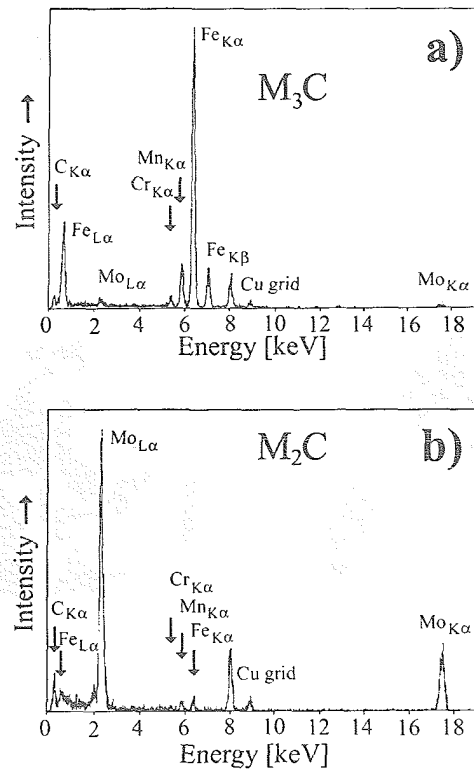
Figure 5 Characteristic EDX-spectra of M_3C (a) and M_2C (b) carbides.
