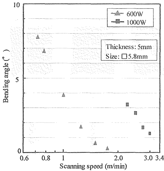
Fig. 12 Bending angle dependency on beam power
