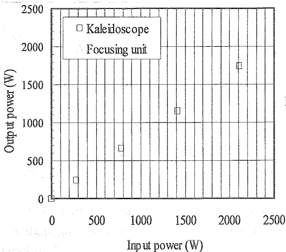
Fig. 5 Efficiency of the kaleidoscope
