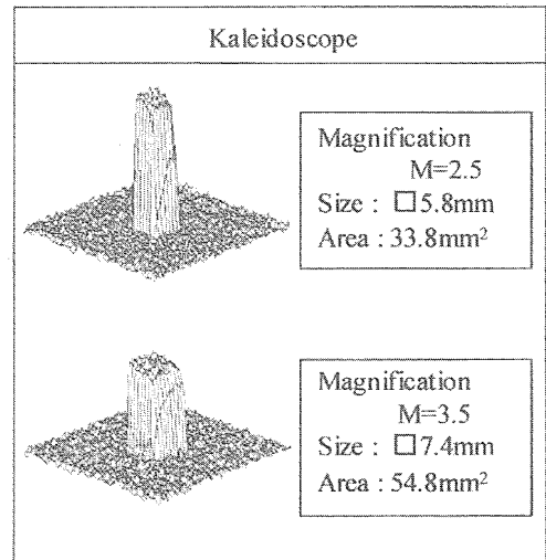
Fig. 4 Beam profiles with kaleidoscope
