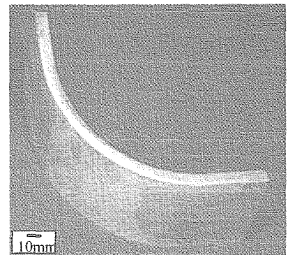
Specimen: SUS304 Thickness: 10mm Power: 950W Scanning speed : 0.54m/min Laser scan: 10 × 36
