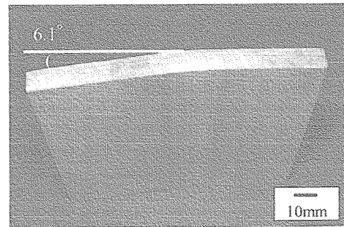
Laser Power: 1000W Material: SUS304 Thickness: 10mm Scanning Speed: 1.0m/min Number of laser Scans: 50
