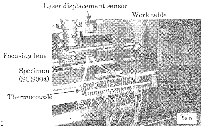
Fig. 6 Experimental setup
