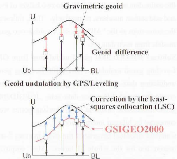
Fig. 4 Schematic diagram of hybrid geoid model construction.
