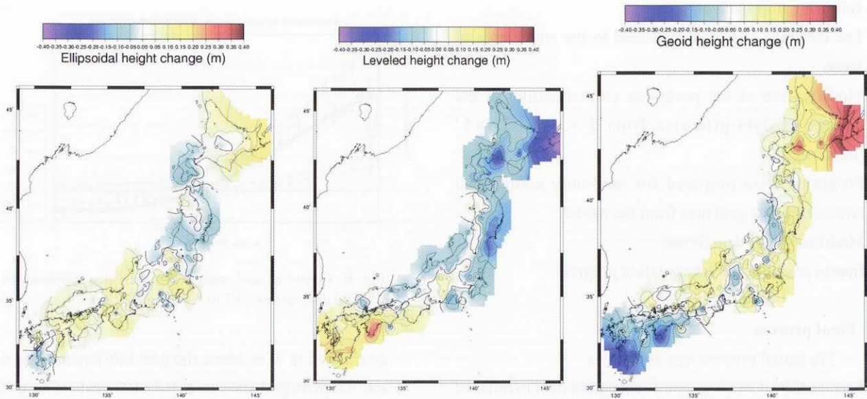
Fig. 3 The difference between the old and new analyses for GPS ellipsoidal heights (left), leveled heights (middle) and geoid undulation data (right). Color scale is -0.4\text{m} to 0.4\text{m} . Contour interval is 5\text{cm} and broken lines show contours of negative value.
