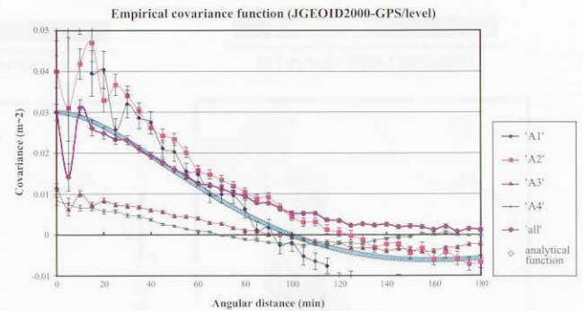
Fig. 6 Empirical and analytical covariance functions of geoid differences. A1 to A4 denote local areas.
