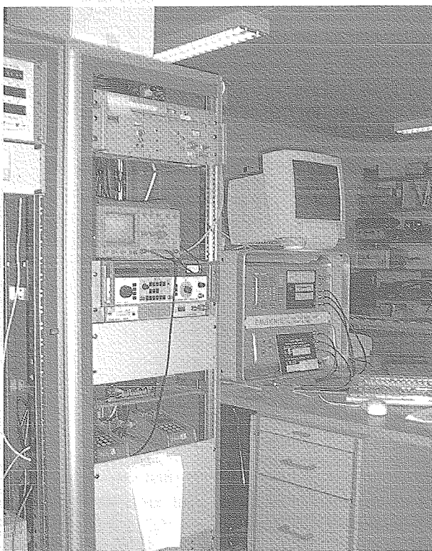
Fig. 7. The Lowell ionosonde. The Lowell unit itself is beneath the computer monitor. The rack to the left contains frequency reference equipment including synchronisation with nearby instruments (Photo: Bjørnar Hansen).
