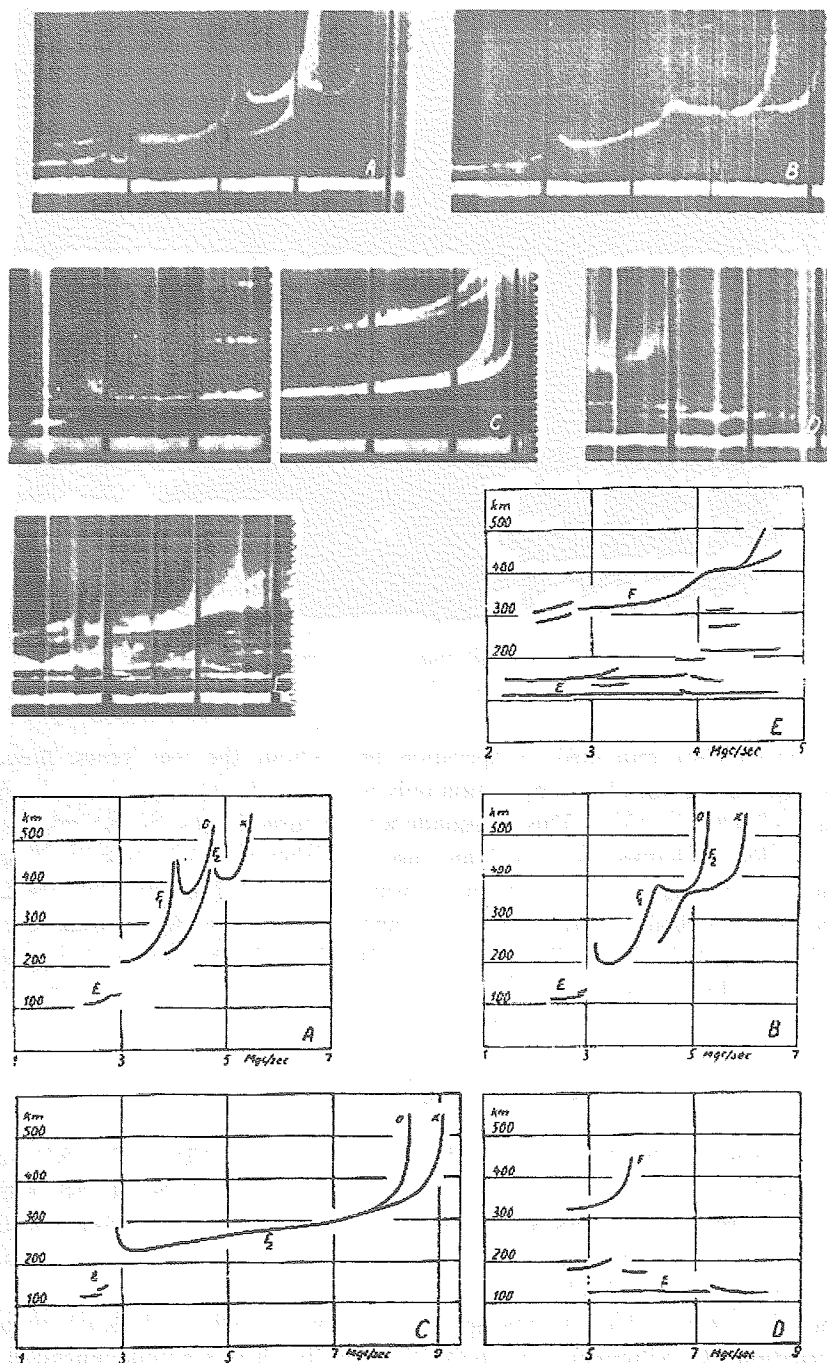
Fig. 3. Early results from the first Norwegian ionosonde on a variety of days between May 1935 and October 1936. The line drawings show the operators' interpretations of the echoes, and, importantly the calibrations necessary for any re-analysis of the archived photographic recordings (Harang, 1937).
