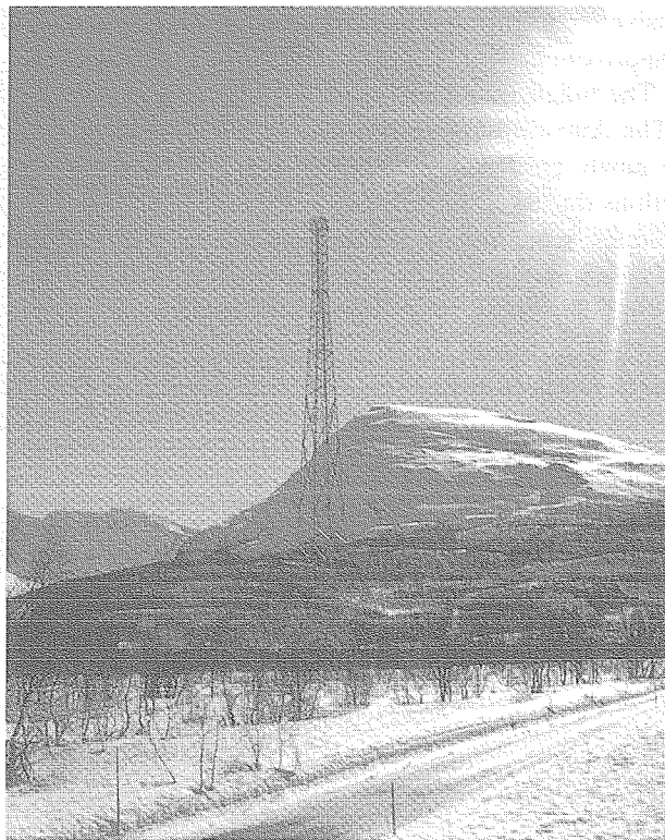
Fig. 8. The current transmitter antenna arrangement at Ramfjordmoen (Photo: Chris Hall).
