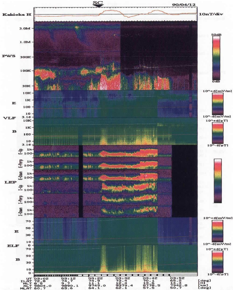
Fig. 4. Example of an SC event occurring at 0325:52(UT) on April 12, 1990, when the Akebono satellite passed through the cusp region. The formats of the PWS, VLF and ELF spectra are the same as in Fig. 4. The fifth to tenth panels show the LEP data of the electrons and ions for the pitch angles of three sectors and an energy range of 10 eV to 20 keV. In the LEP spectra, 'E-Up', 'E-Perp', and 'E-Down' indicate the electron spectra for the pitch angle ranges of 0°–60°, 60°–120°, and 120°–180°, respectively, followed by the ion spectra for the same pitch angle ranges as for the electrons. Pitch angles of 0° and 180° correspond to the downward and upward directions along the magnetic field line, respectively, since the Akebono satellite is located in the northern hemisphere. In the ELF spectra, the white line shows the proton cyclotron frequency. The enhancement of whistler mode plasma waves and particle fluxes in association with the SC is shown.
