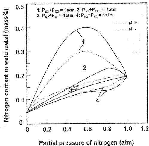
Fig.5 Effect of partial pressure of nitrogen in various carrier gases on the nitrogen absorption of stainless steel weld metal in MIG welding.
