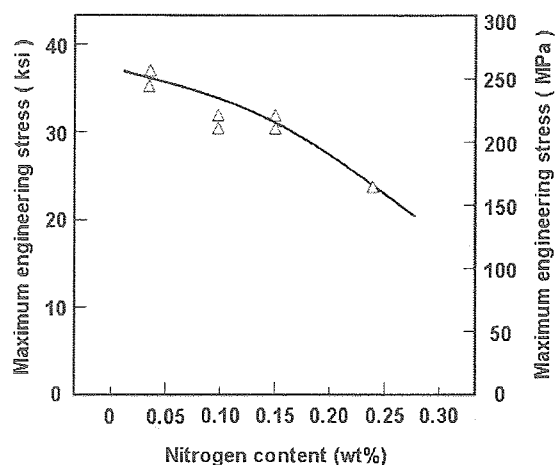
Fig.15 Maximum engineering stress vs. wt% nitrogen for type 304 weld metal specimens tested in boiling \text{MgCl}_2 .
