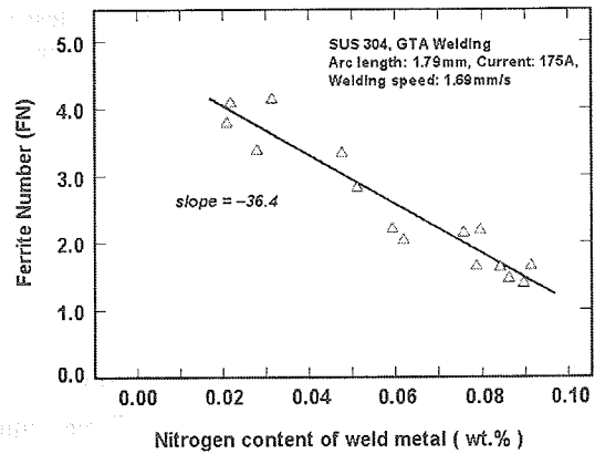
Fig.10 Ferrite number as a function of weld metal nitrogen content.
