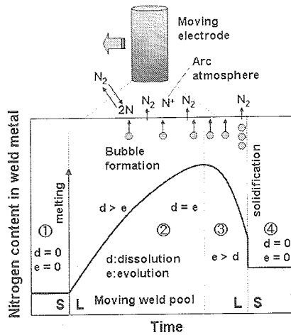
Fig.2 Schematic illustration of the weld metal nitrogen content under a moving welding arc in an atmosphere-containing nitrogen gas (N 2 ): Stage 1: premelting stage, Stage 2: arc melting with dissolution dominating. Saturation (i.e., d=e) may or may not be reached. Note that d=e is a time independent condition and not necessarily a thermodynamic equilibrium condition, Stage 3: Weld metal cooling (still liquid) with decreasing saturation solubility and evolution dominating (bubble evolution may prevail), Stage 4: Solidification with step change in solubility and consequent rejection of nitrogen with excess causing porosity, accompanying nitrogen in solid solution.
