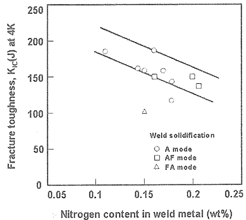
Fig.17 Effects of nitrogen content and solidification mode on the fracture toughness, K_{IC}(J) , of the GTA welds at 4K.
