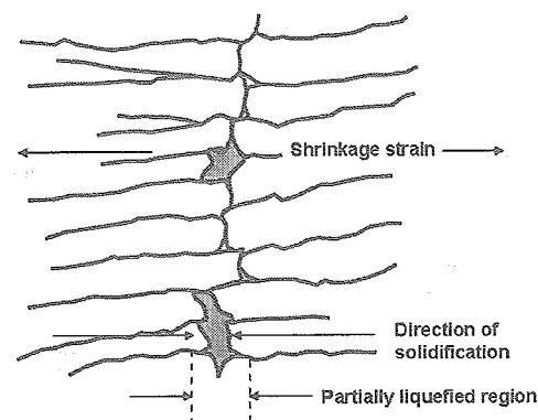
Fig.11 Schematic illustration of mechanism for solidification cracking.
