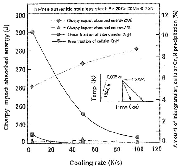
Fig.18 Effect of cooling rate on Charpy impact absorbed energy and amount of intergranular, cellular Cr 2 N precipitation.
