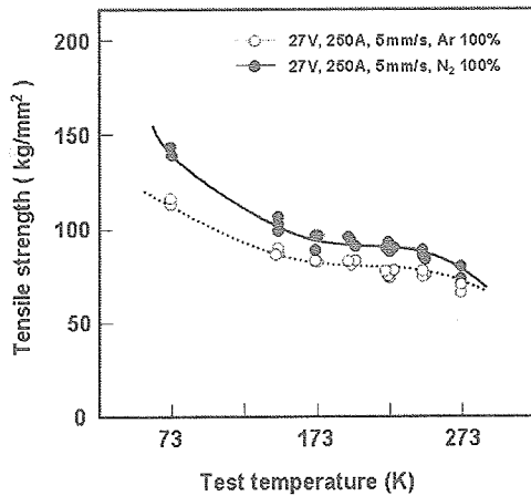
Fig.16 Effect of temperature on the tensile strength of SUS 316 welds made in N_2 shielding gas.
