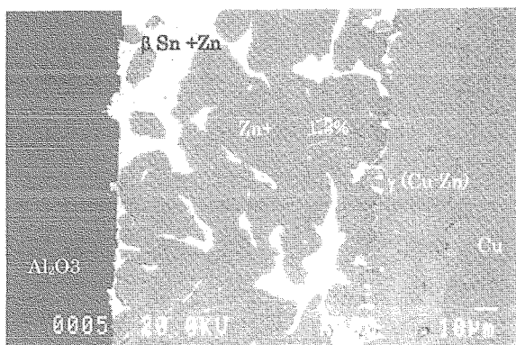
Fig. 3 SEM micrograph of Al 2 O 3 /30Sn-70Zn/Cu interface
