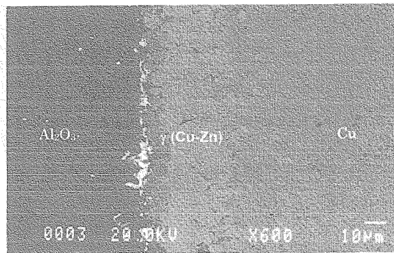
Fig. 5 SEM micrograph of Al 2 O 3 /60Sn-40Zn/Cu interface
