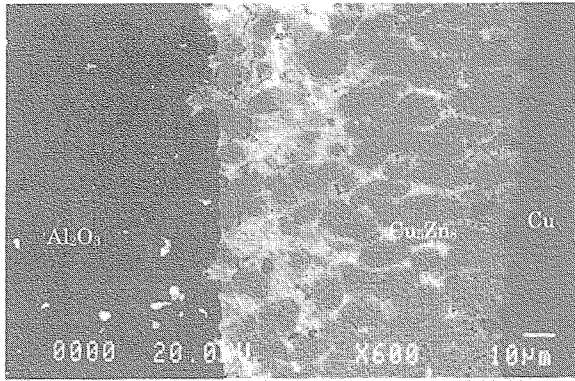
Fig. 7 SEM micrograph of Al 2 O 3 /91Sn-9Zn/Cu interface
