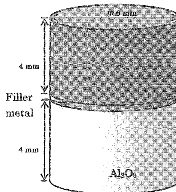
Fig. 2. Specimen after joining.
