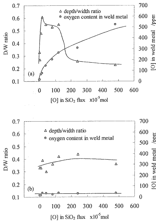
Fig. 5 D/W ratio and oxygen content in weld vs. SiO 2 flux quantity (a) 4μm (b) 25μm
