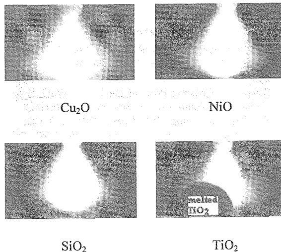
Fig.9 Arc images in welding with different flux
