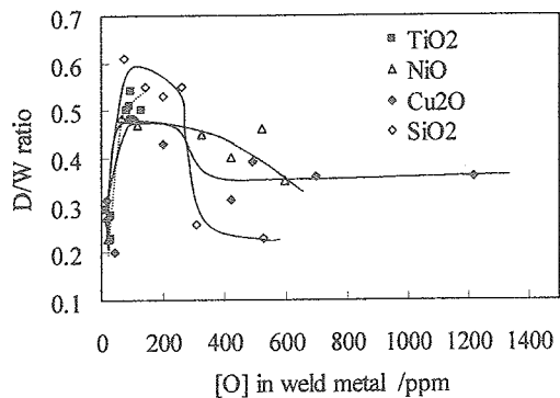
Fig.8 D/W ratio vs. [O] in weld metal
