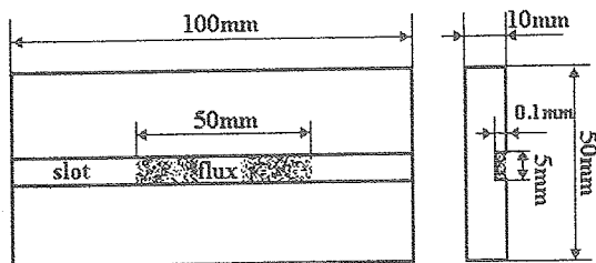
Fig.1 Schematic of the SUS304 plate used in GTAW
