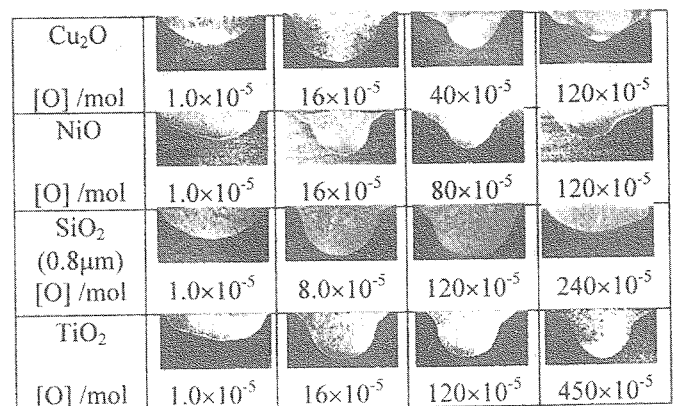
Fig. 2 Weld cross-sections with different oxides 2mm
