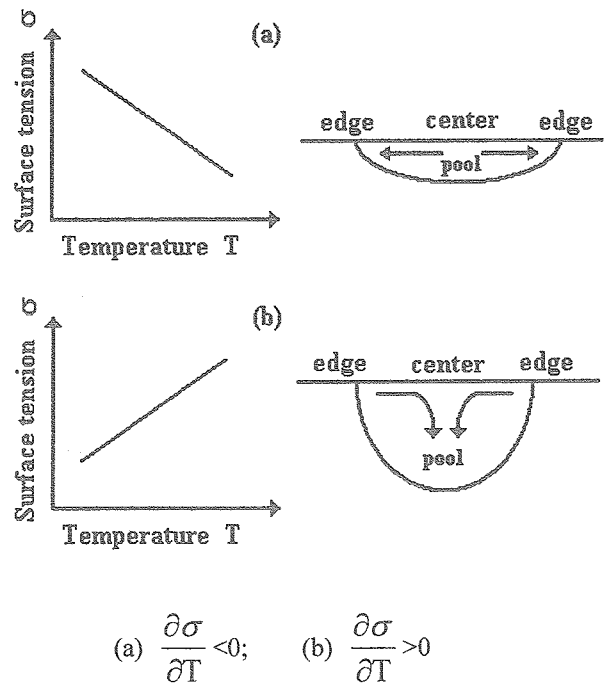
Fig.6 Marangoni convection mode by surface tension gradient
