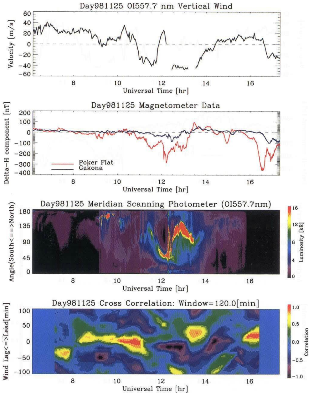
Fig. 2. Case 1: November 25, 1998. A comparison of the vertical wind as deduced from the Doppler shift of OI557.7nm with the CRLFPI (top panel), \Delta H -component of the magnetic field (second panel) and the temporal variation of OI557.7nm auroral location as obtained with the Meridian Scanning Photometer (third panel). The bottom panel shows the correlation between the vertical wind and magnetic variation as obtained at Poker Flat. The vertical axis indicates the time difference (positive value: wind leading), and the degree of correlation is presented as the color code.
