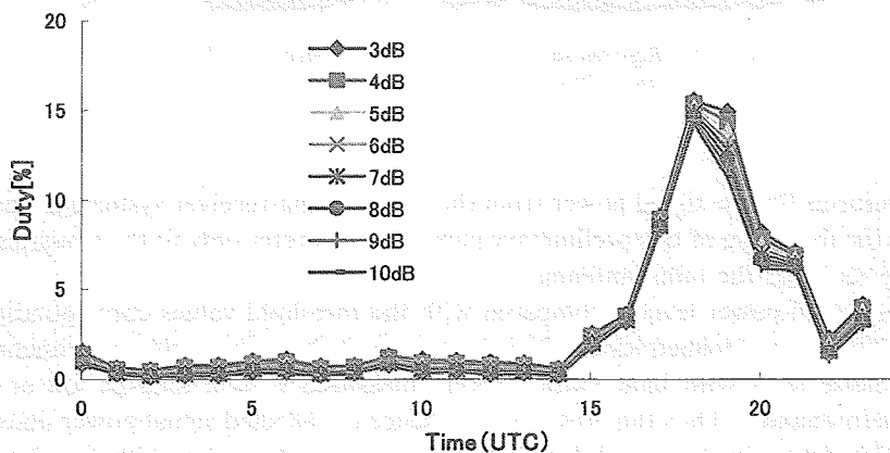
Fig. 7. Average duty cycle vs. time of day (Averaged over April 1st–30th, 2002).
