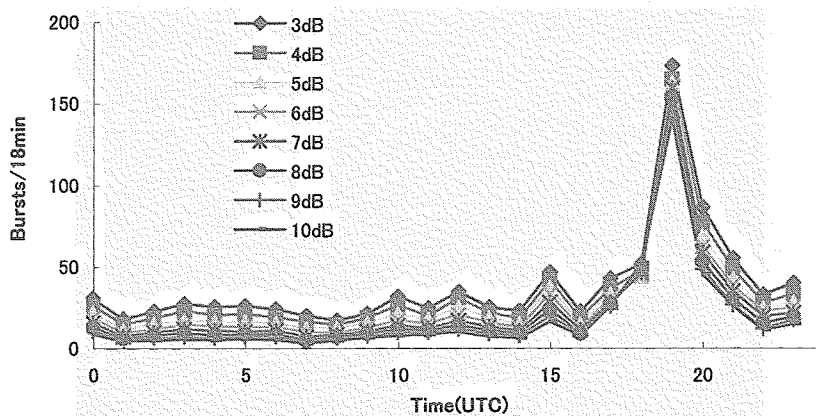
Fig. 6. Average number of bursts vs. time of day (Averaged over April 1st–30th, 2002).
