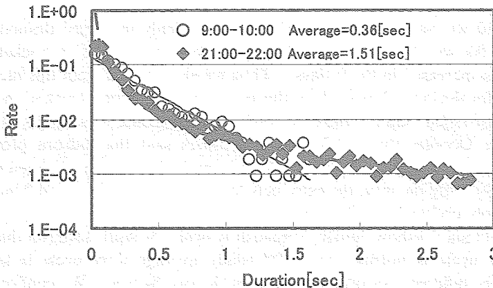
Fig. 9. Comparison of the distribution (relative frequency) of duration of the channel between meteoric (9 h to 10 h) and non-meteoric (21 h to 22 h) hours (April 1st–September 30th, 2002).
