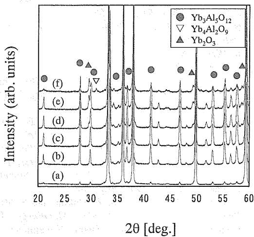
Fig. 3 XRD patterns of millimeter-wave-sintered aluminum nitrides with (a)1wt%, (b)2wt%, (c)3wt%, (d)4wt%, (e)5wt%, and (f)6wt% \text{Yb}_2\text{O}_3 .
