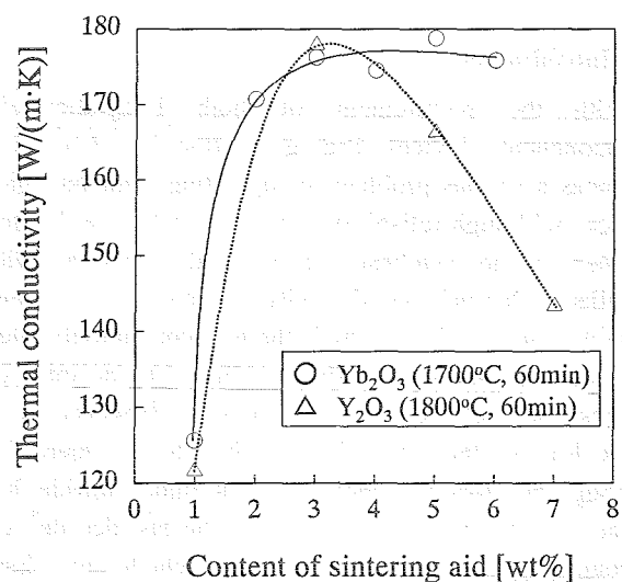
Fig. 2 Dependence of thermal conductivity of millimeter-wave-sintered aluminum nitrides on the content of sintering aid.
