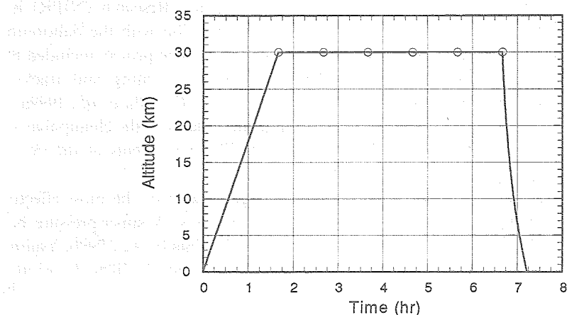
Fig. 1. Time-altitude profile used in trajectory calculation. Small circles indicate one-hour intervals after a ceiling altitude is reached.
