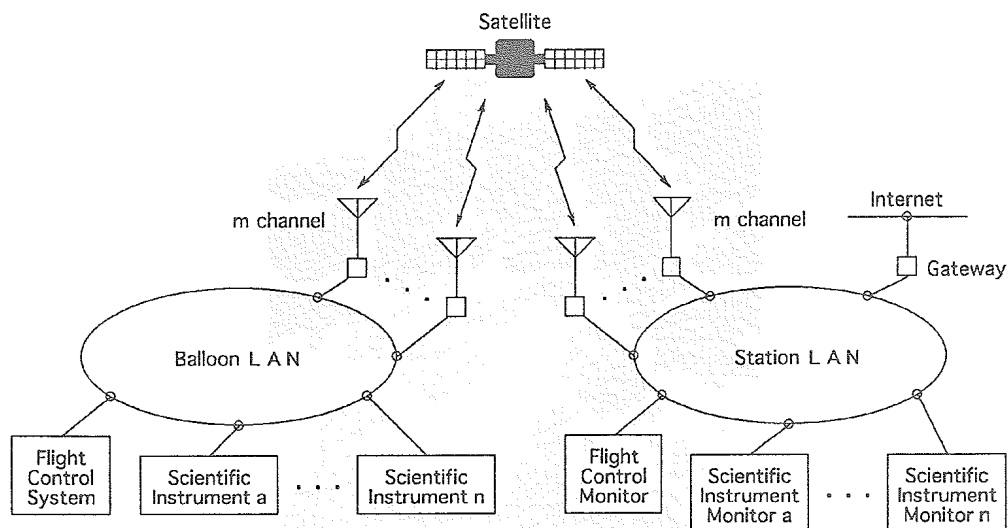
Fig. 7. Schematic diagram of a network configuration onboard the balloon, a telecommunications system, a ground station and Internet connections.
