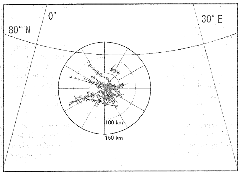
Fig. 4. Trajectories of June 1995 superimposed on a map of Ny-Alesund. The three large circles indicate the distance from the launch pad, 50 km, 100 km and 150 km, respectively. Small circles on each trajectory present the same time and altitude as in Fig. 1.
