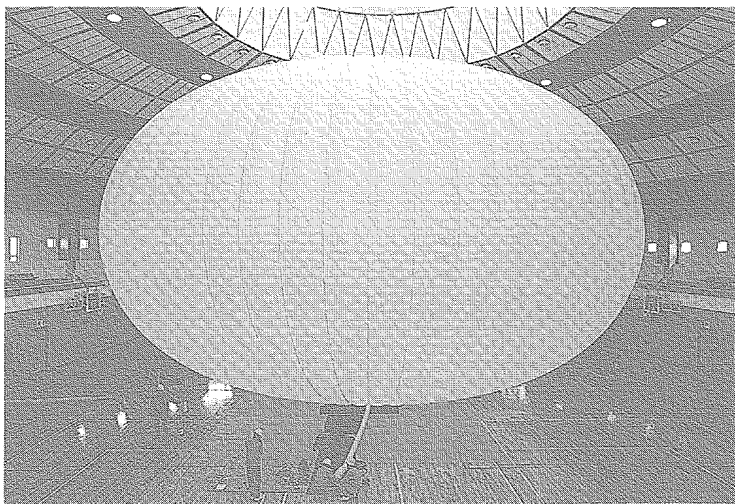
Fig. 6. A 3000 m 3 super-pressure balloon under an indoor inflation test.
