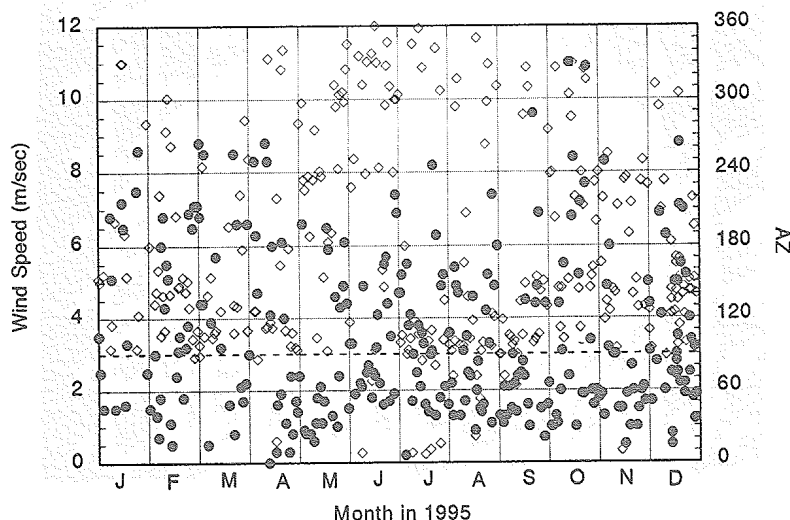
Fig. 5. Surface wind speed (black circles) and direction (white boxes) distribution at Ny-Ålesund in 1995. The broken line of 3 m/s indicates the maximum wind speed for safe launching of large balloons.
