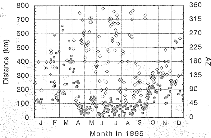
Fig. 2. Simulated landing point distances (black circles) and directions (white boxes) distribution from the launch pad in Ny-Ålesund, 1995. AZ indicates the direction, 0, 90 and 180 are north, east and south, respectively.
