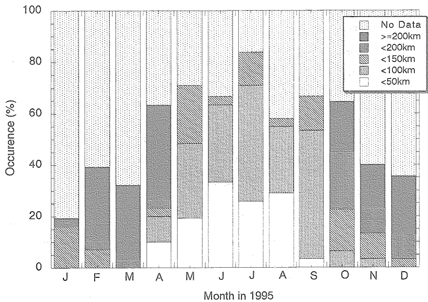
Fig. 3. Occurrence of simulated landing point distances, as shown in Fig. 2, classified into six categories. <100 km includes landing point distances of at least 50 km but less than 100 km, for example. "No data" means that the calculation was not performed because no meteorological data were available or the balloon burst altitude was lower than 28 km.
