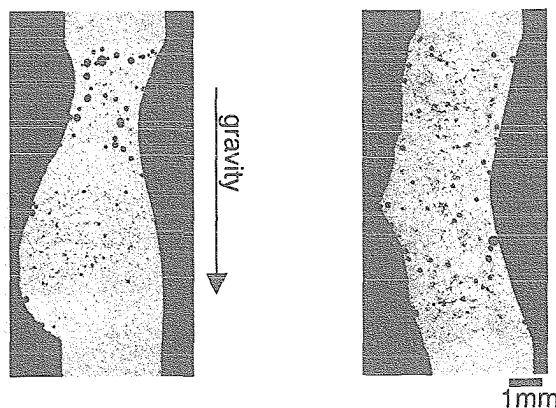
Fig.7 Transverse sections of bead-on-plate welds in horizontal welding with argon-1% hydrogen mixed shielding gas.
