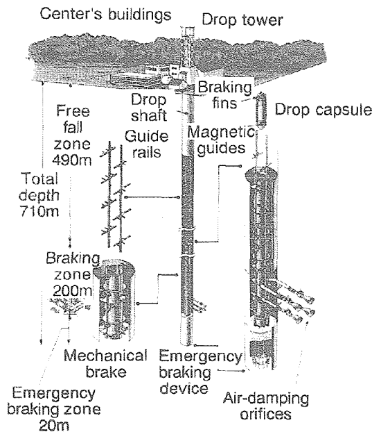
Fig.1 Schematic illustration of the free fall system.
