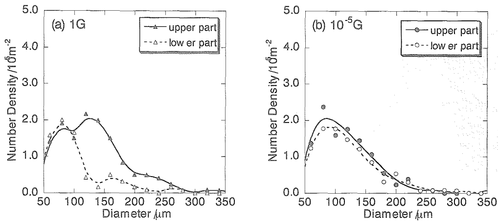
Fig.9 Blowhole size distributions separated the results in Fig.8 (a).
