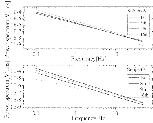
Fig.7 Approximate curve in fluctuation characteristics (top: subject A, bottom: subject B, both logarithmic axes).
