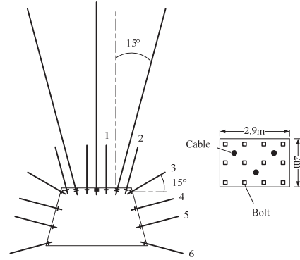
Fig.1 Layout of bolt and cable
