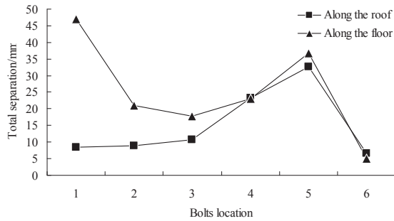
Fig.5 Total separation between two measuring points close to bolt junction
