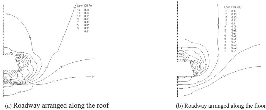
Fig.3 Total-displacement-contour map of surrounding rock
