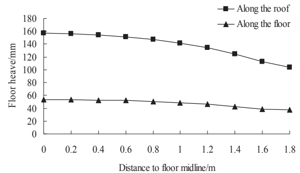
Fig.4 Floor heave of measuring points
