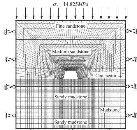
Fig.2 Numerical model
