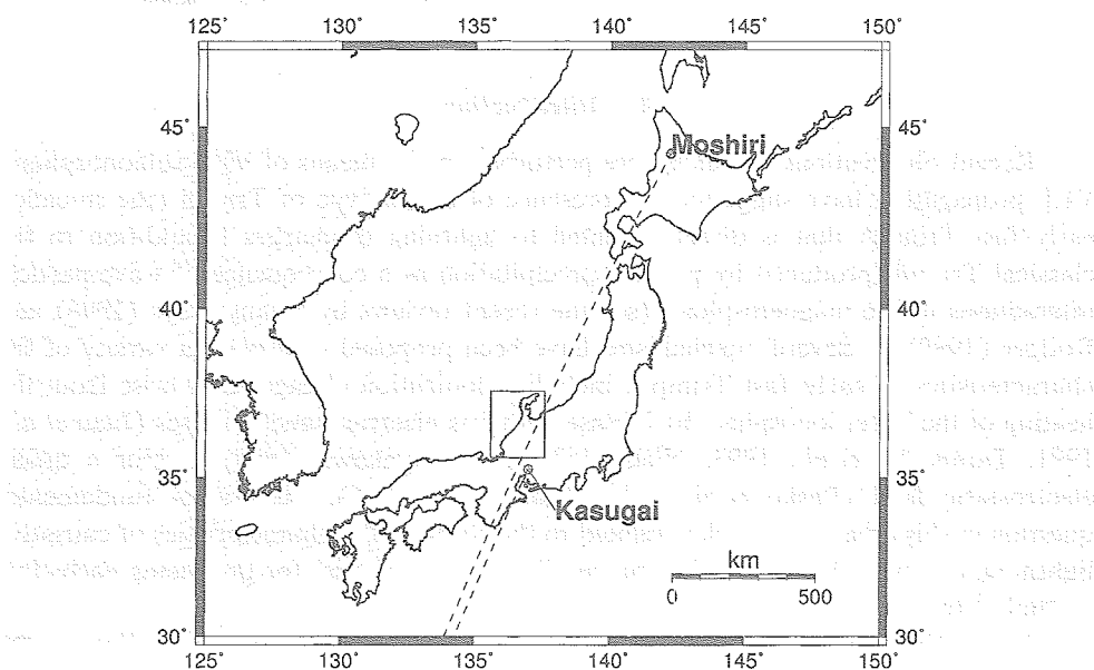
Fig. 1. Locations of two observation stations (Moshiri and Kasugai), together with the great circle path to the VLF transmitter of NWC (Australia). The rectangle indicates the area of interest.
