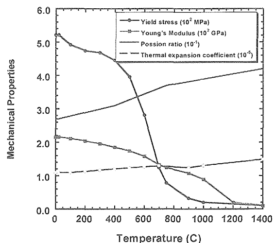
Fig. 4 Temperature dependent thermal mechanical properties.
