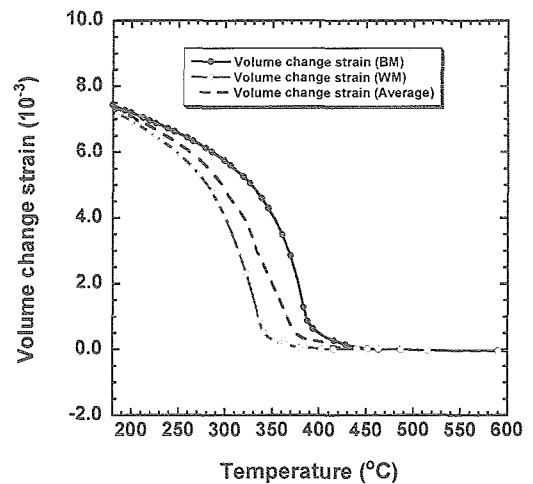
Fig. 7 Volumetric change of modified 9Cr-1Mo steel.
