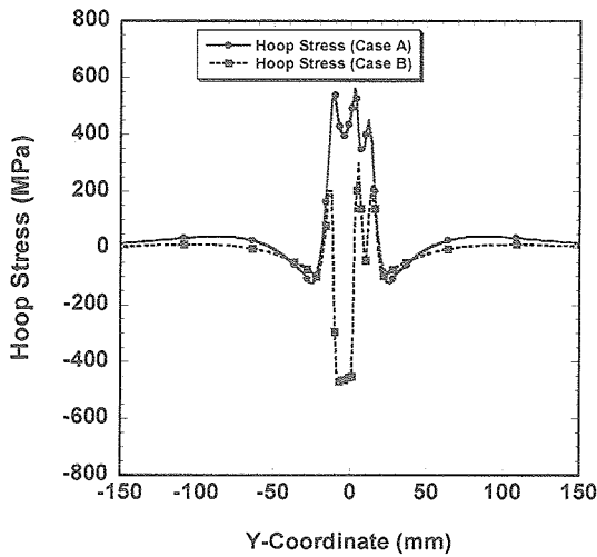
Fig. 9 Hoop stress distributions of case A and case B on the outer surface.
