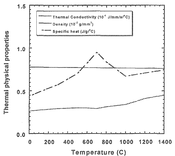
Fig. 3 Temperature dependent thermal physical properties.
