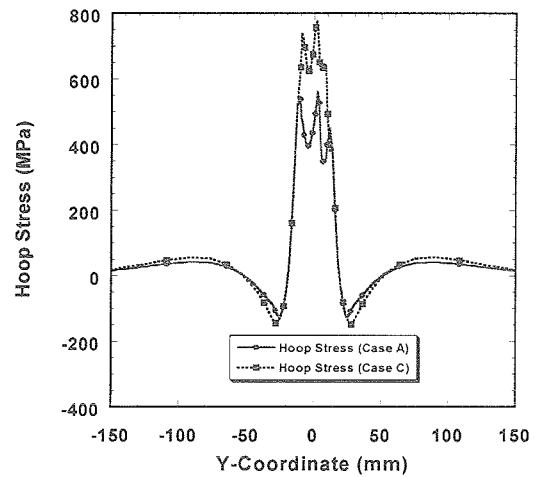
Fig. 11 Hoop stress distributions of case A and case C on the outer surface.
