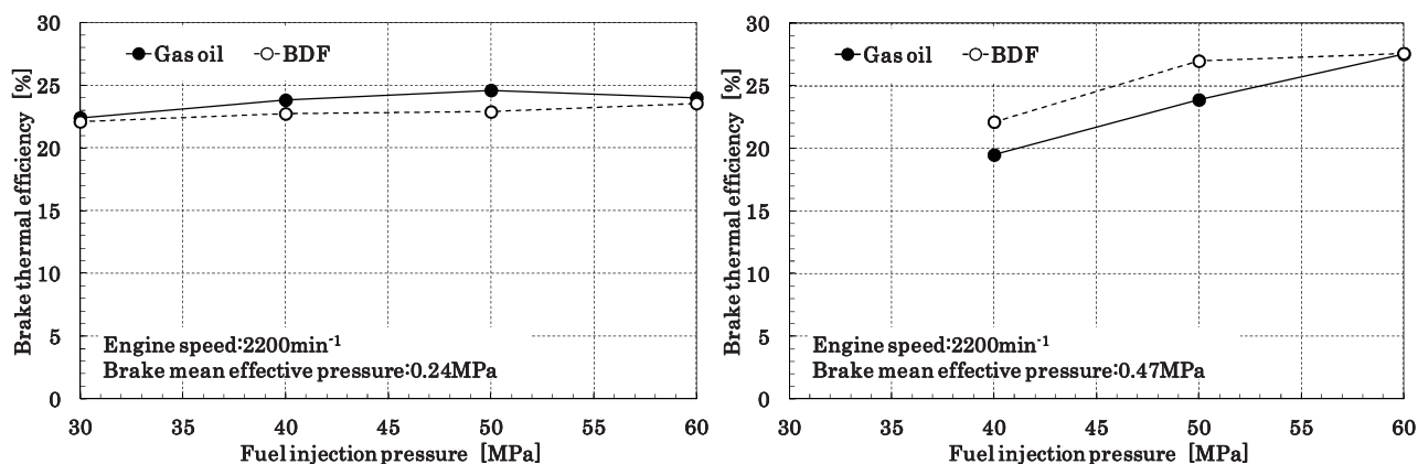
Fig. 1 Variations of brake thermal efficiency with fuel injection pressure measured by using gas oil and BDF for the brake mean effective pressures 0.24MPa (left) and 0.47MPa (right)
