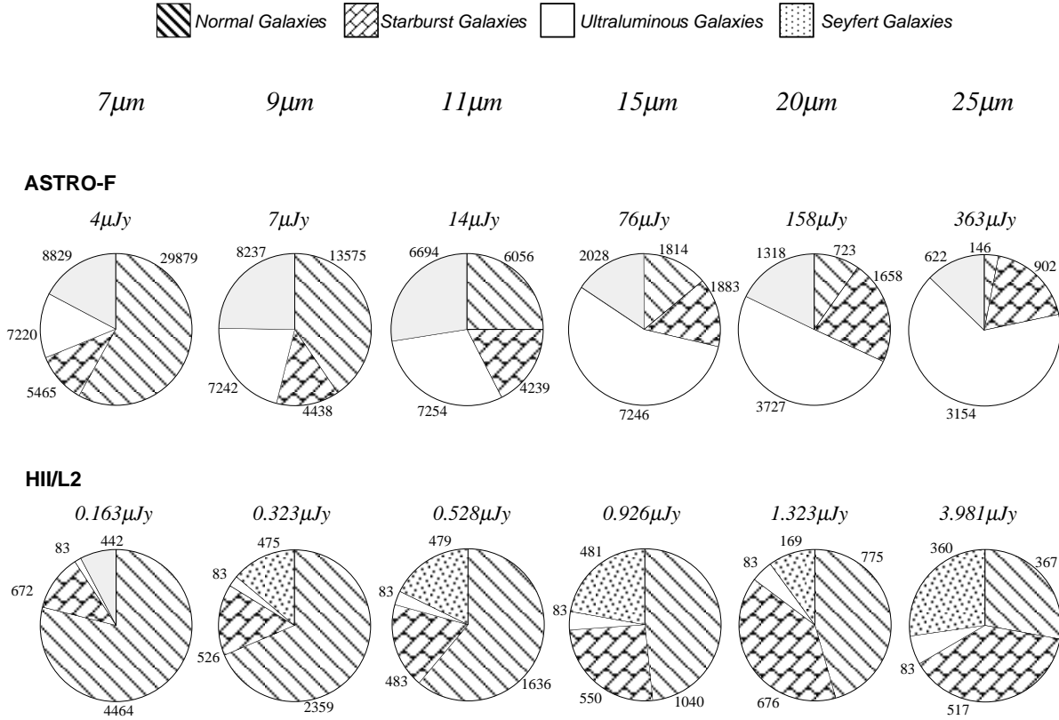
Fig. 2: Summary of ASTRO-F deep 3200sq.arcmin. ( top ) and HII/L2 0.01sq.deg. ( bottom ) Mid-IR surveys. Predicted numbers and relative proportions of galaxies are shown for the respective survey sensitivity limits (in \mu Jy ) in Table 2. Note that if the survey sensitivity is source confusion limited then the sensitivity limit is dependent on the evolutionary model.
