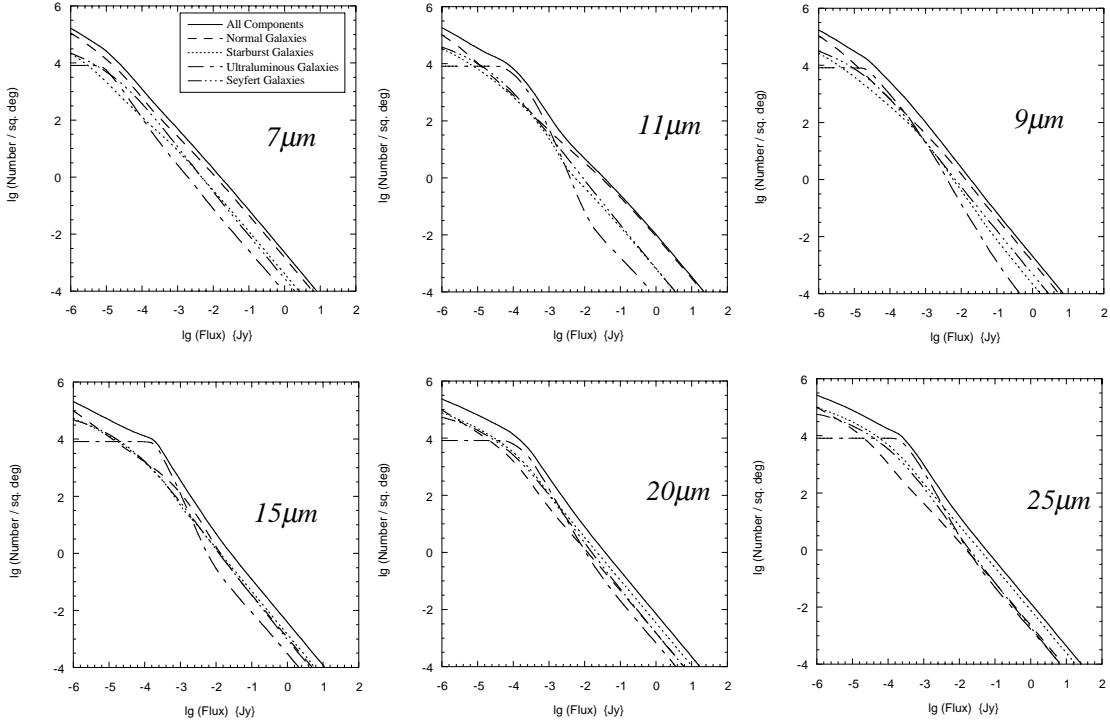
Fig. 1: Integral galaxy source counts, as described in the text, at 7, 9, 11, 15, 20 & 25 \mu\text{m} respectively, corresponding to the IRC-MIR-S and IRC-MIR-L filter wavelengths. Total source counts are shown ( solid line ) with normal ( dash ), starburst ( dot ), ultraluminous galaxy ( dash dot ) and AGN components ( dot-dot-dot-dash ).
