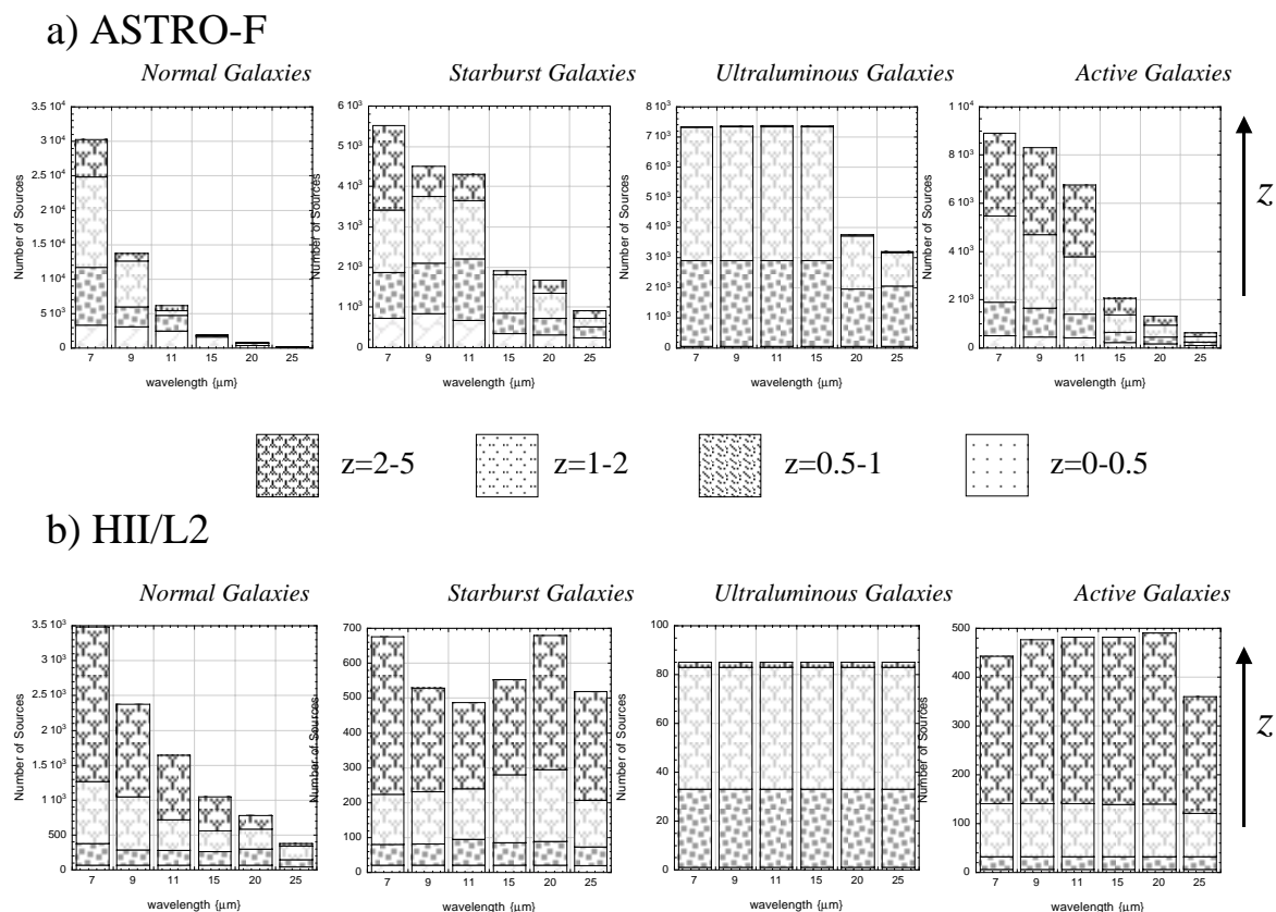
Fig. 3: N-z distributions for ASTRO-F deep 3200sq.arcmin. ( top ) and HII/L2 0.01sq.deg. ( bottom ) mid-IR surveys. Predicted numbers and relative proportions of galaxies are shown for the respective survey sensitivity limits (in mJy ) in Table 2. Note the scales on the axes differ
