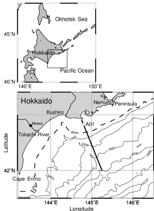
Figure 2-1. Bathymetry off the southeastern Hokkaido, Japan. Dashed line indicates 200m depth isobath line. Thick line and open circle (A01) denote the regular observational line, which is called the A-line, for cross sections of Figs.2-11 - 2-14, and observational point for Fig. 2-17, respectively. The closed circle labeled with “Moiwa” indicates observational point of river discharge at a downstream site of the Tokachi River (Fig. 2-16)
