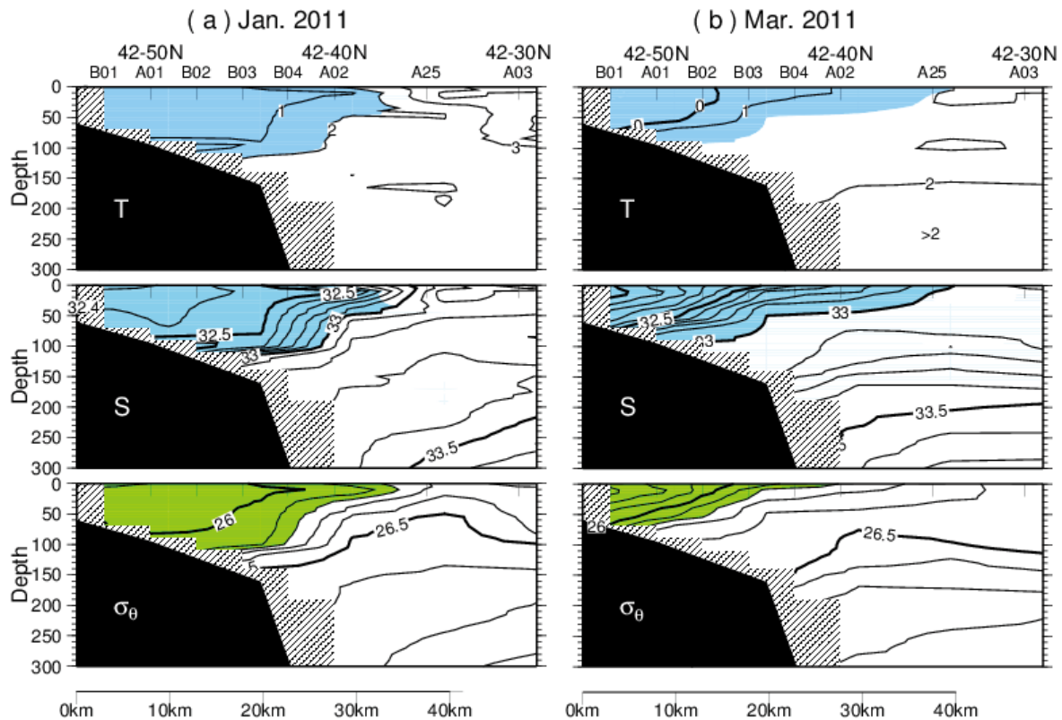
Figure 4-9. Vertical cross-sections of temperature [ ^{\circ}\text{C} ], salinity and potential density [ \sigma_{\theta} ] across the transect B01-A03 (Fig. 4-1) in January (a) and March (b) 2011, respectively. Light blue-shaded regions in each upper and middle panel and yellow green-shaded regions in each lower panel denote COW ( T < 2^{\circ}\text{C} and S < 33 ) and lower density region than 26.2\sigma_{\theta} , respectively. Obliquely hatched regions in each figure denote no data
