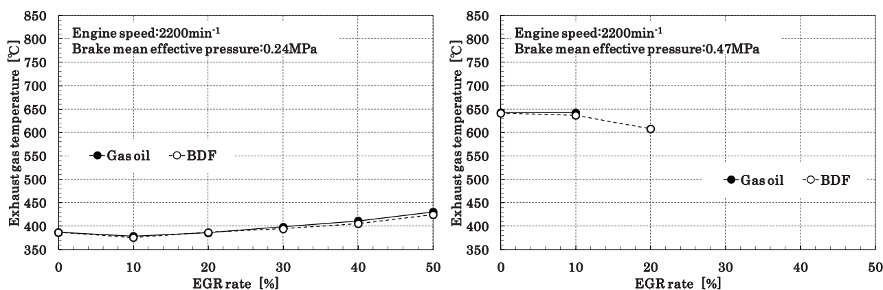
Fig. 3 Variations of exhaust gas temperature with EGR rate measured by using gas oil and BDF for the brake mean effective pressures 0.24MPa (left) and 0.47MPa (right)
