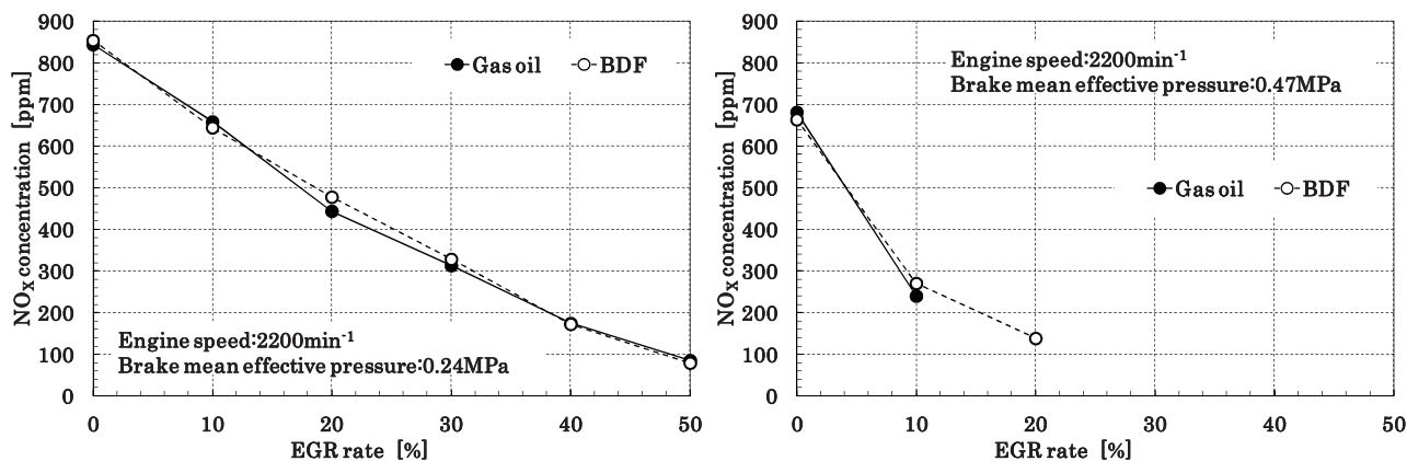
Fig. 2 Variations of \text{NO}_x concentration with EGR rate measured by using gas oil and BDF for the brake mean effective pressures 0.24MPa (left) and 0.47MPa (right)
