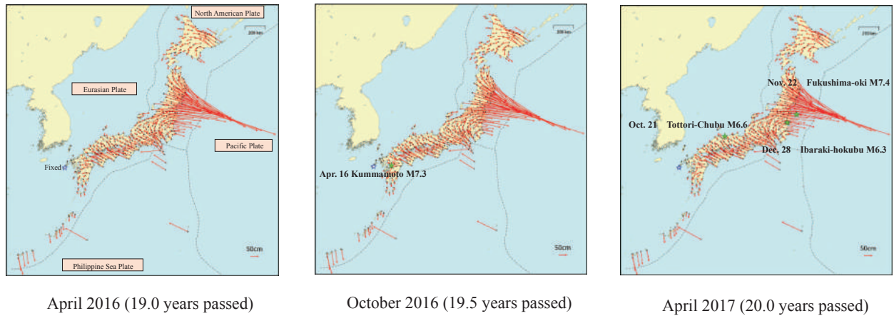
Figure 6 Crustal deformations in Japan for every half years from April 1997 (from April 2016 to April 2017)
