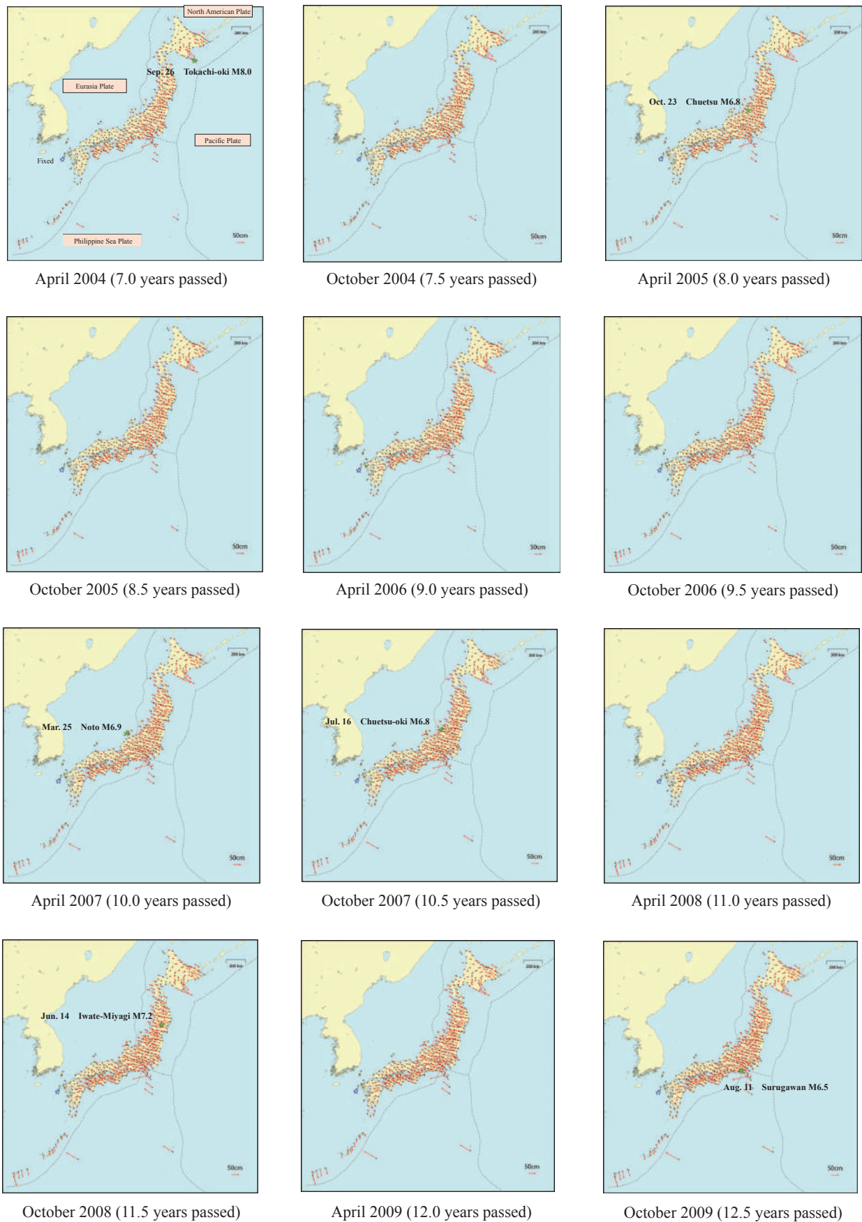
Figure 4 Crustal deformations in Japan for every half years from April 1997 (from April 2004 to October 2009)
