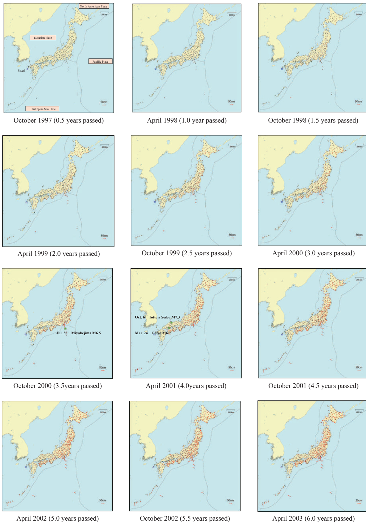
Figure 3 Crustal deformations in Japan for every half years from April 1997 (from October 1997 to April 2003)
